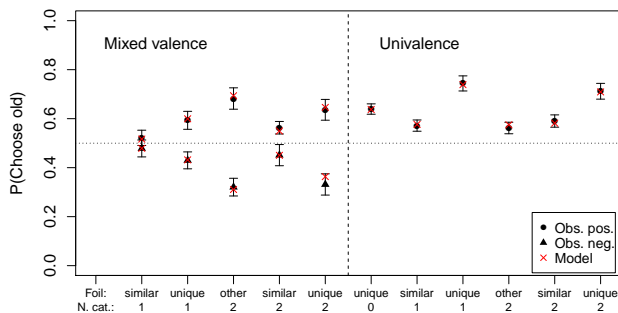
Figure 3: Data and predictions for Experiment 1.
