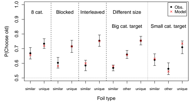
Figure 4: Data and predictions for Experiment 2.
